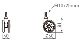
CMF60BB-1PC-T14 (non-brake)
