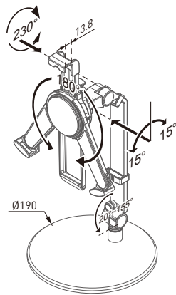
TA-131 desk stand
