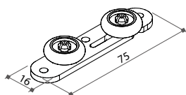
56990T Double Roller Top Gear
