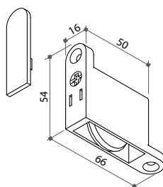
56990CF Bottom Running Gear, center fixing
