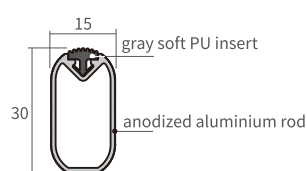
SECTION
