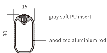
SECTION
